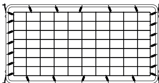
D Mattress Support
